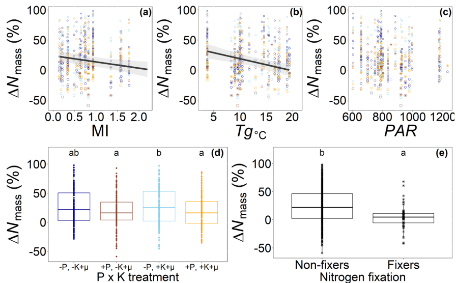
FIGURE 4 | Scatter plots depicting the relationship between (a) \Delta N_{\text{mass}} and global moisture index (MI), (b) between \Delta N_{\text{mass}} and growing season temperature ( T_g ), and (c) between \Delta N_{\text{mass}} and photosynthetically active radiation (PAR) (c). Box plots depicting the (d) variation of \Delta N_{\text{mass}} depending on P and \text{K}_{+\mu} treatments, and (e) \text{N}_2 -fixation capacity. Significant linear regressions (a and b) are represented by the regression lines derived from a linear mixed-effects model, with \Delta N_{\text{mass}} as the dependent variable and soil P and \text{K}_{+\mu} treatments, MI, T_g , PAR, photosynthetic pathways, and \text{N}_2 -fixation capacity as fixed effects. Shaded regions around the regression lines represent 95% confidence intervals. Larger dots indicate higher \Delta N_{\text{mass}} . Star dots indicate \text{N}_2 -fixers, while circle dots indicate non-fixers. Dark blue dots indicate treatments which did not receive P and \text{K}_{+\mu} , brown dots indicate treatments which received P but not \text{K}_{+\mu} , blue light indicate treatments which received \text{K}_{+\mu} but not P, and orange dots indicate treatments which received P and \text{K}_{+\mu} . The lettering above each box indicates groupings based on post hoc Tukey's tests, where different letters denote statistically different groups at \alpha = 0.05 across all groups shown.
