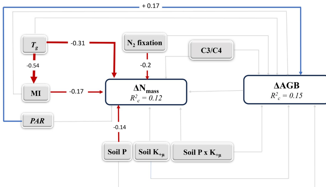
FIGURE 5 | Structural equation model illustrating the interaction between \Delta \text{AGB} and \Delta N_{\text{mass}} and disentangling the direct and indirect effects of climatic variables, soil nutrient treatments, photosynthetic pathways, and N_2 -fixation on \Delta N_{\text{mass}} through its covariance with \Delta \text{AGB} . Path coefficients are depicted as simple standardised regression coefficients. The width of connections indicates estimates of standardised path coefficients, with solid lines denoting significant connections and semi-transparent lines indicating non-significant connections. Negative relationships are depicted by red lines. Positive relationships are depicted by blue lines. R^2 for component models is given in the boxes of response variables and is reported as the conditional R^2 ( R^2_c ) based on the variance of both the fixed and random effects.
